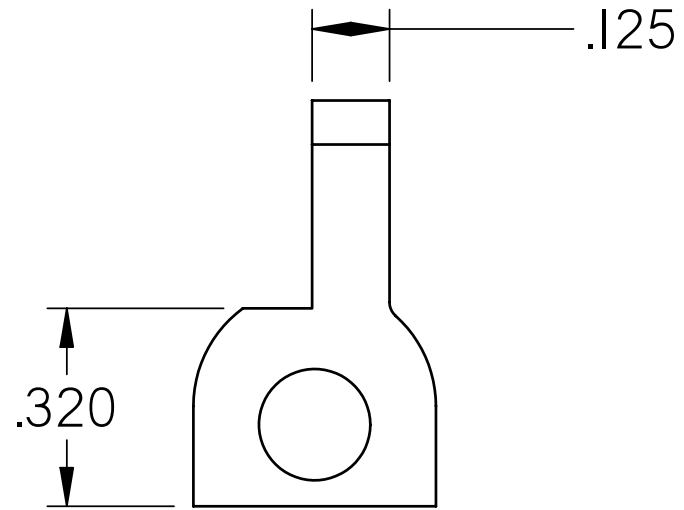
MODIFIED FIRING PIN EXTENSION KEEPER
